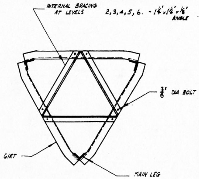
TYPICAL SECTIONS AT LEVELS 2, 3, 4, 5, 6.
