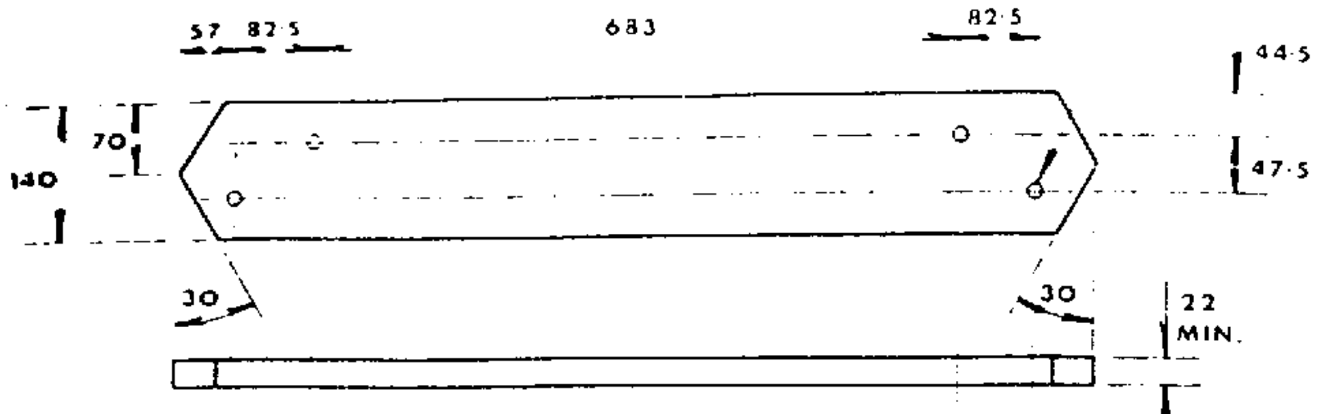
PLATFORM. 3 OFF PER UNIT. MANUFACTURED FROM HARDWOOD.
